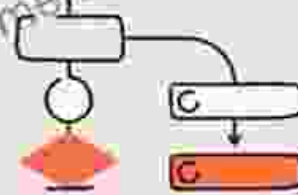
Decision trees
